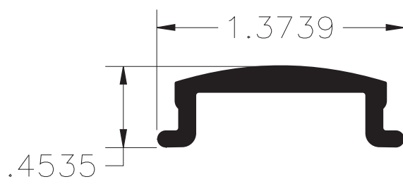
Series 3/4 Radius Filler Part #1201
